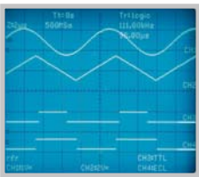
DSO mode: Signal portion expanded with zoom (burst in one line)
